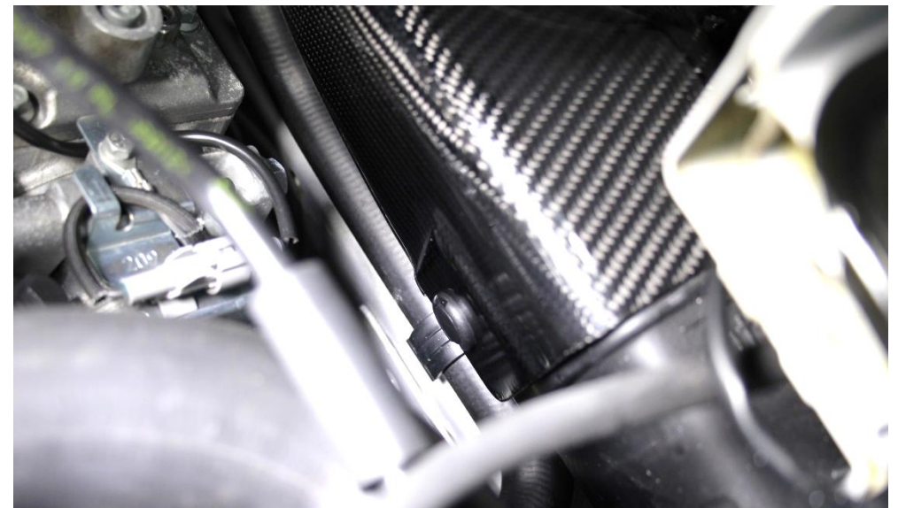
23. Starting on the side closest to the engine - align the hole on the new duct with the hole on the stock opening and push the rivet through. Secure by clicking the head in fully.
