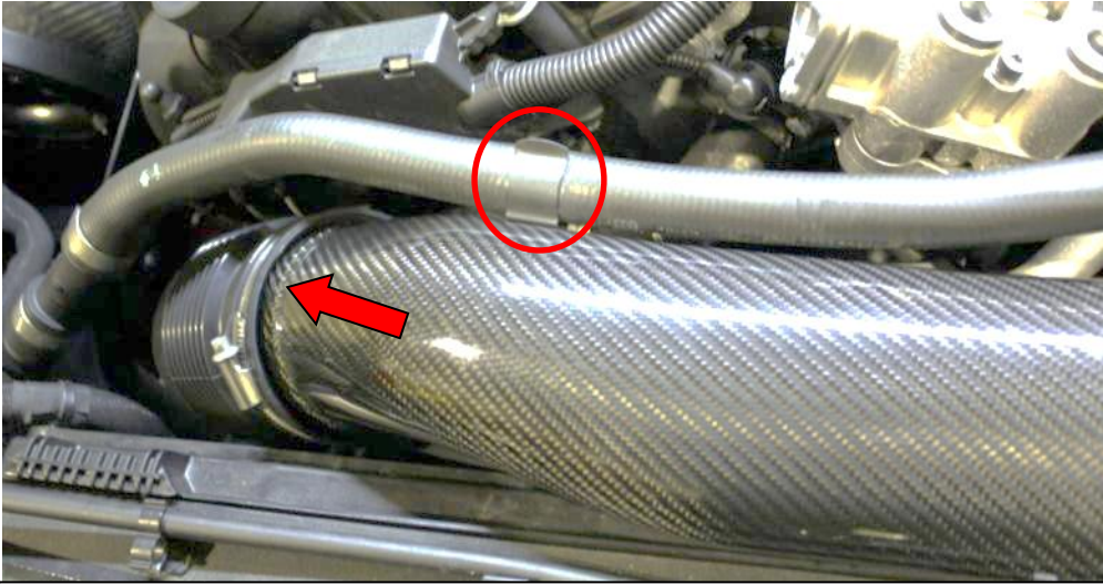
39. Raised section of the carbon tube pushed inside the flexible hose (red arrow). Also push the stock rubber hose into the metal clip on the carbon tube as circled.
